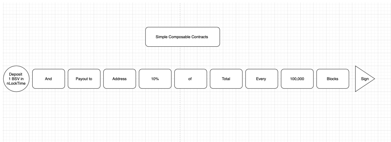
Illustration of a simple composable modular smart contract using nLockTime to pay an annuity every 100,000 blocks
